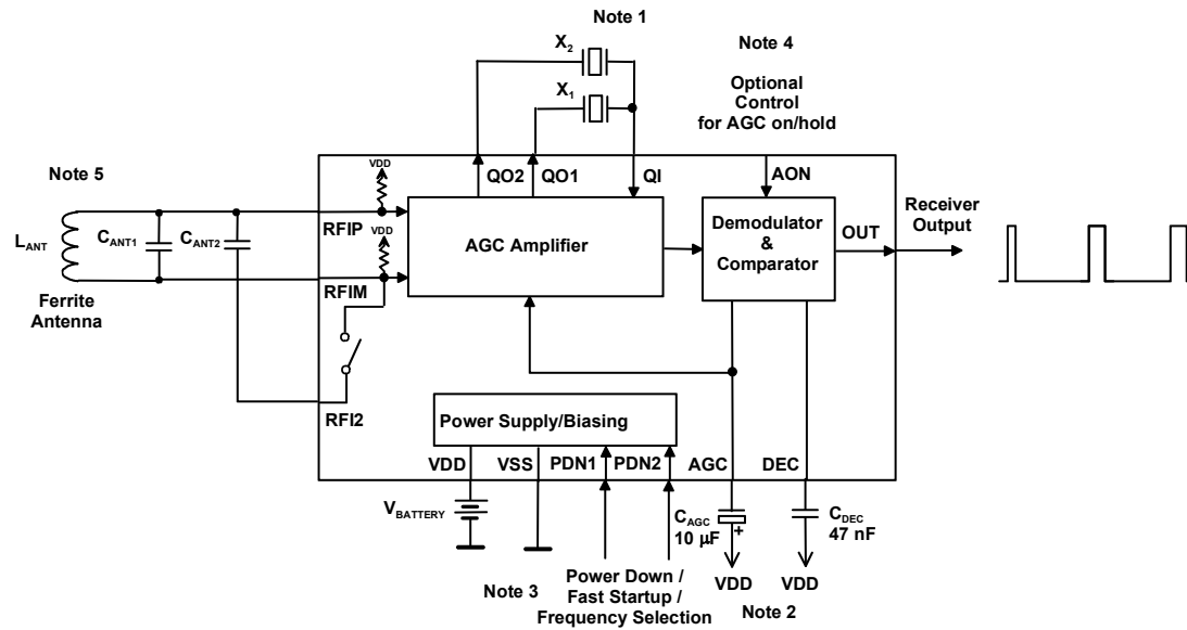
Figure 1. Application circuit of dual band receiver MAS6181
