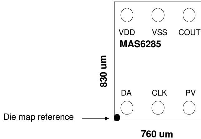
Figure 2. IC outline of MAS6285.
