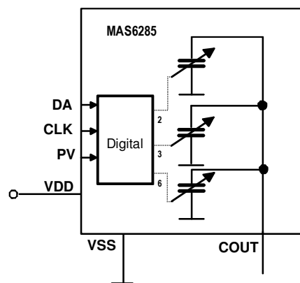
Figure 1. Block diagram of MAS6285.
