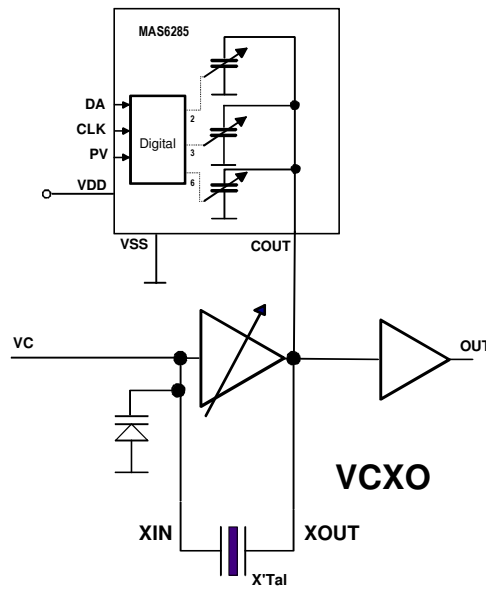
Figure 3. Typical application for MAS6285.
