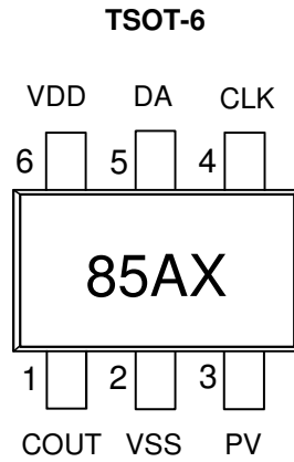
Figure 4. TSOT-6 package.
